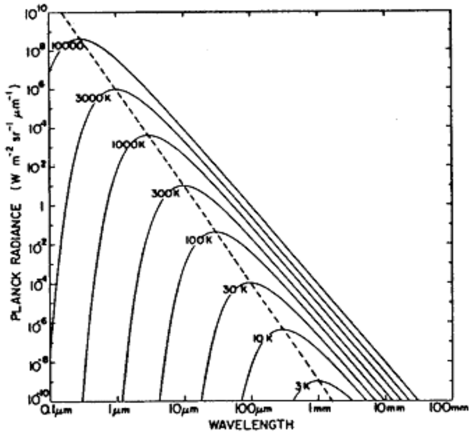
Figure 2.1 Planck function on log-log plot for several temperatures.
