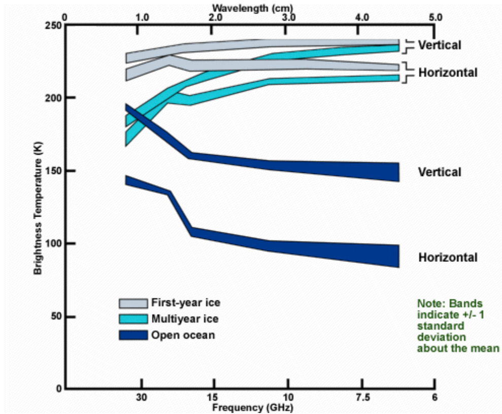
Figure 2.4 Microwave brightness temperature (at vertical and horizontal polarizations) as a function of frequency (wavelength) of first year sea-ice, multiyear sea-ice, and sea water as observed by the Nimbus-7 SMMR (Scanning Multichannel Microwave Radiometer) (Cavalieri et al. 1984).
