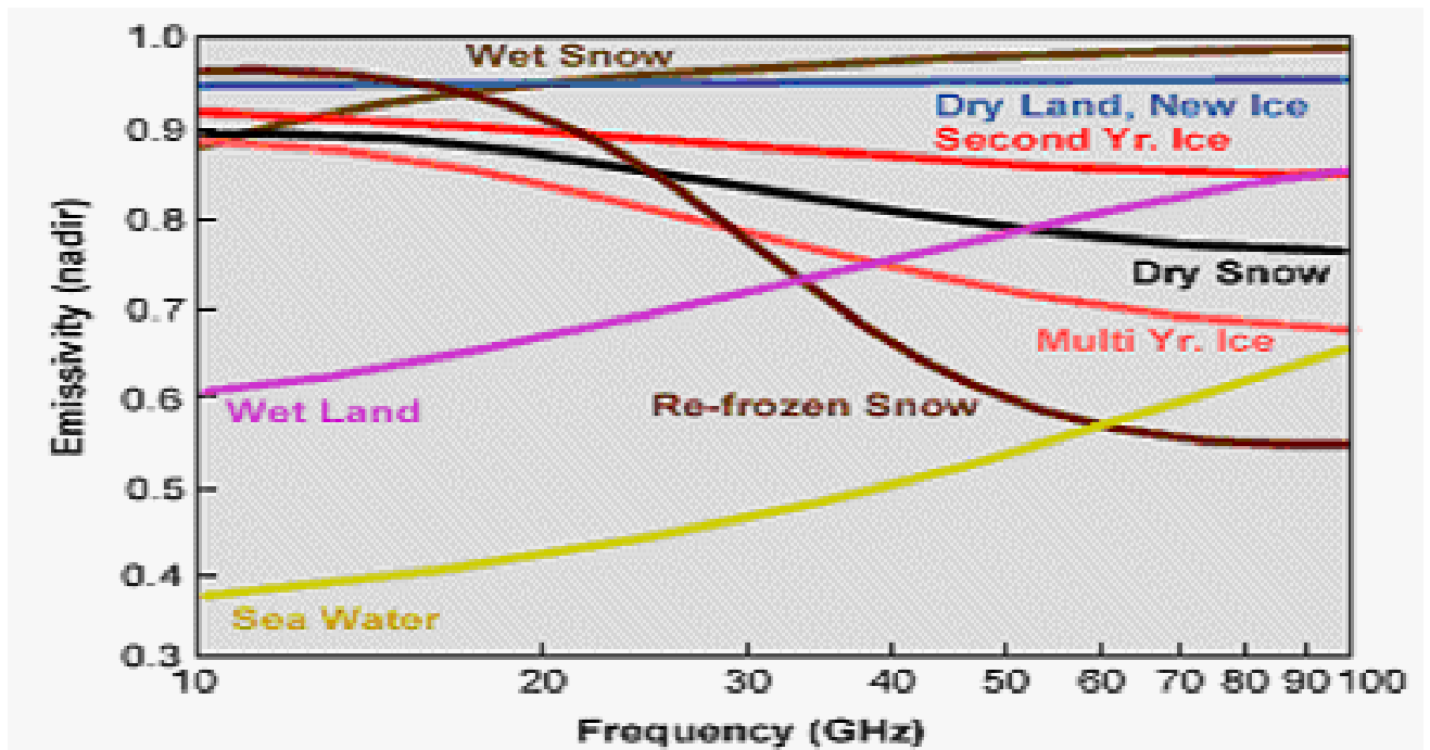
Figure 2.3 Examples of spectral emissivity (at nadir) of some surfaces in the microwave.
