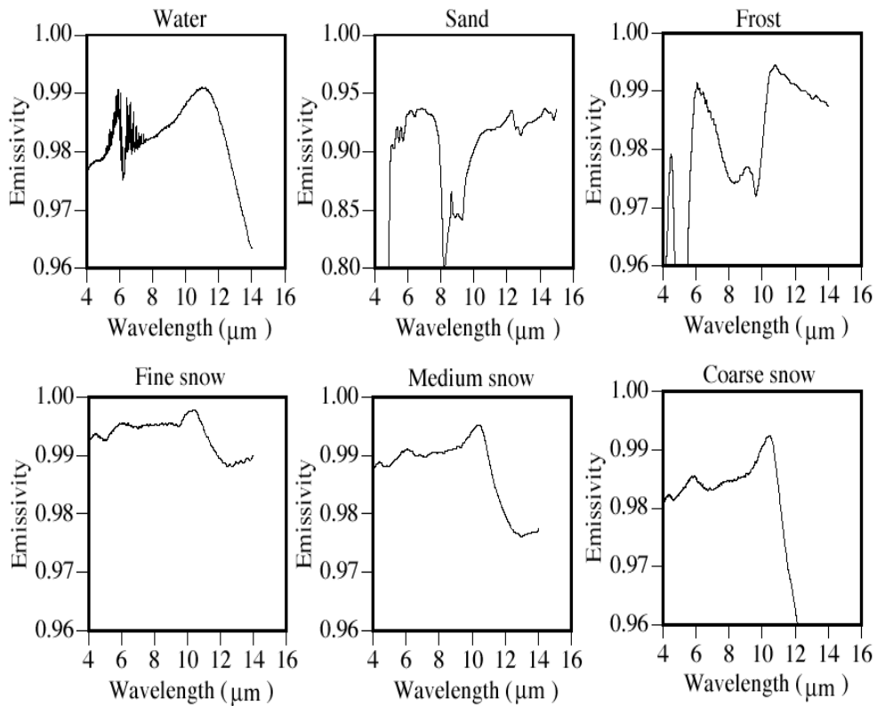
Figure 2.2 Examples of IR spectral emissivity of some surfaces.
