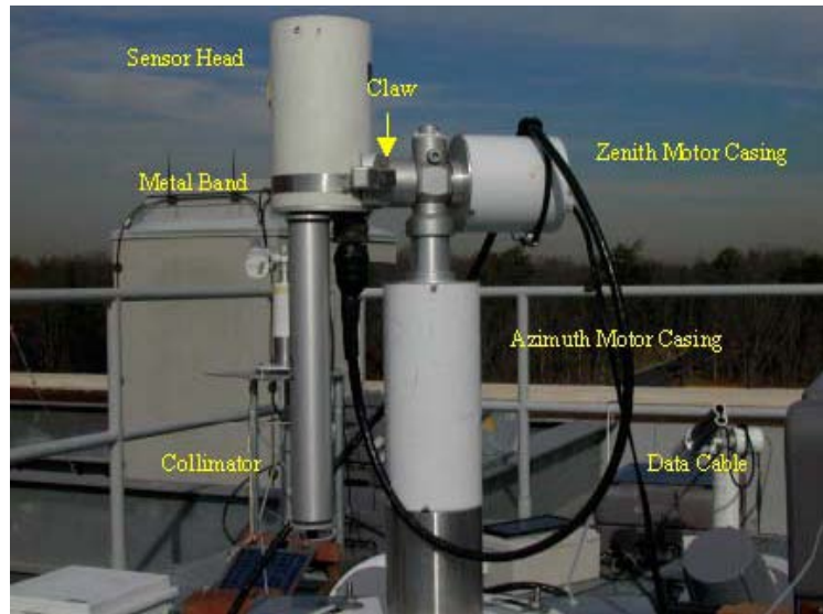
Figure 4.9 Cimel Sunphotometer operated by AERONET. Typical spectral bands (channels) of the Cimel sunptometer (central wavelengths): 340 nm, 380 nm, 440nm, 500 nm, 675 nm, 870 nm and 1020nm.
