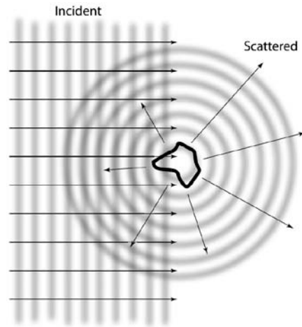
Figure 4.1 Simplified visualization of scattering of an incident EM wave by a particle.
