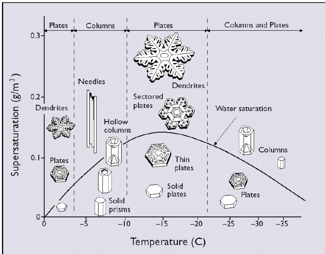
Figure 4.3 Ice crystal's shape as a function of supersaturation and temperature – a “classical” view
