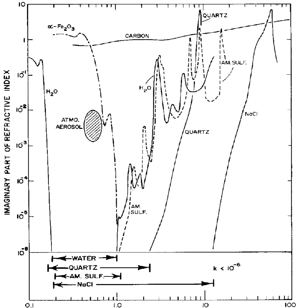
Figure 4.6 “Classical plot” of the imaginary part of the refractive indexes of some aerosol materials as a function of wavelength (in \mu\text{m} ) (Bohren and Huffman, Fig.5.16).
