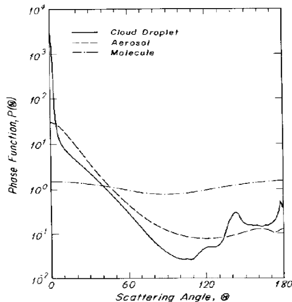
Figure 4.8 Examples of representative scattering phase functions (at a wavelength of 0.5 \mu\text{m} ) for aerosol and clouds particles. The molecular (Rayleigh) is also shown for comparison.
