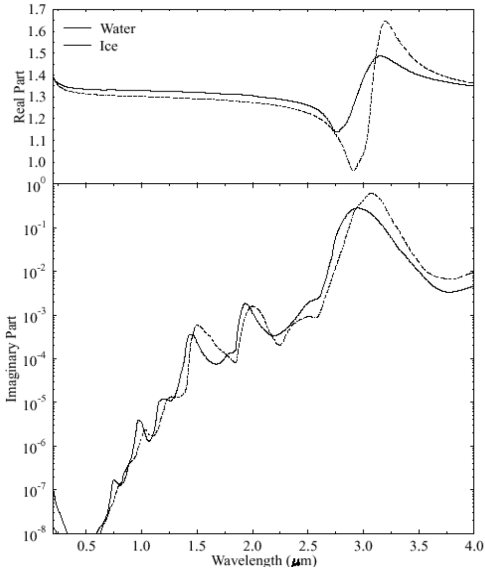
Figure 4.4 The refractive index of water and ice in the visible and near-IR.
