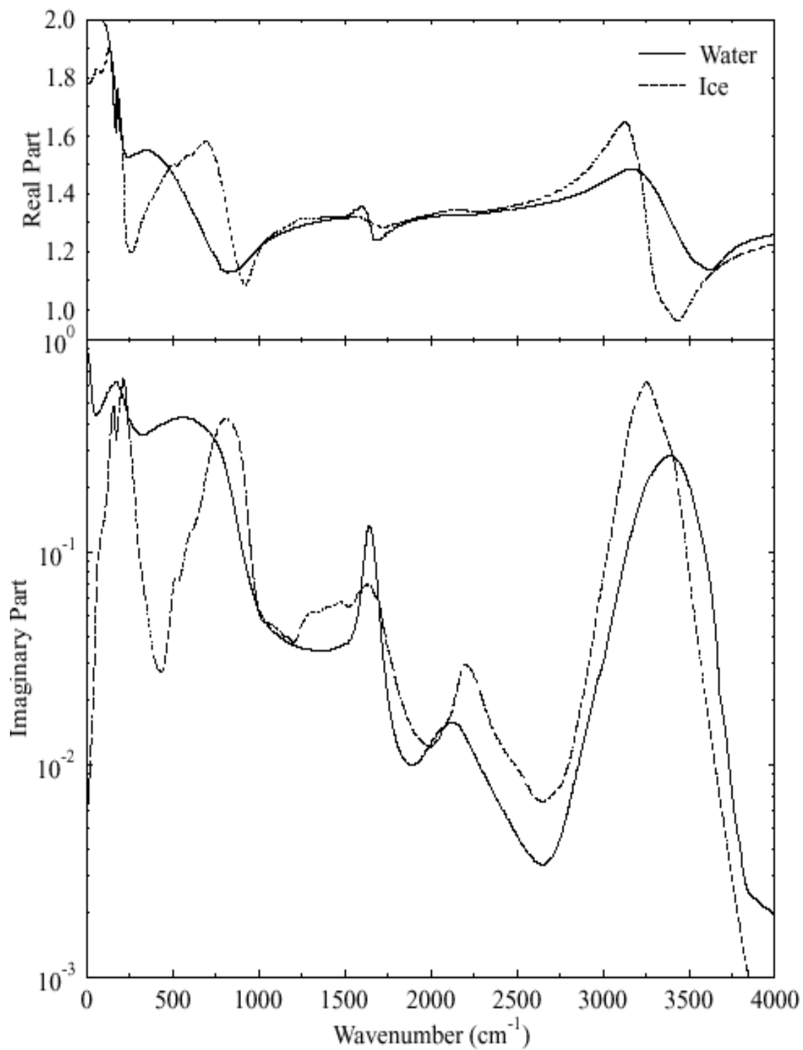
Figure 4.5 The refractive index of water and ice in the IR.
