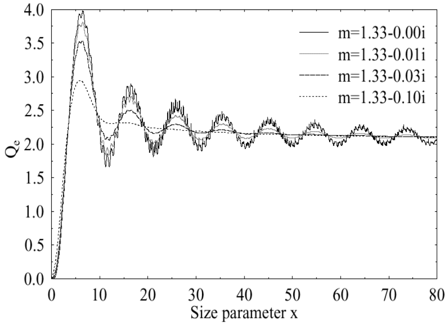
Figure 4.7 Examples of Q_e calculated with the Mie theory for several refractive indexes.
