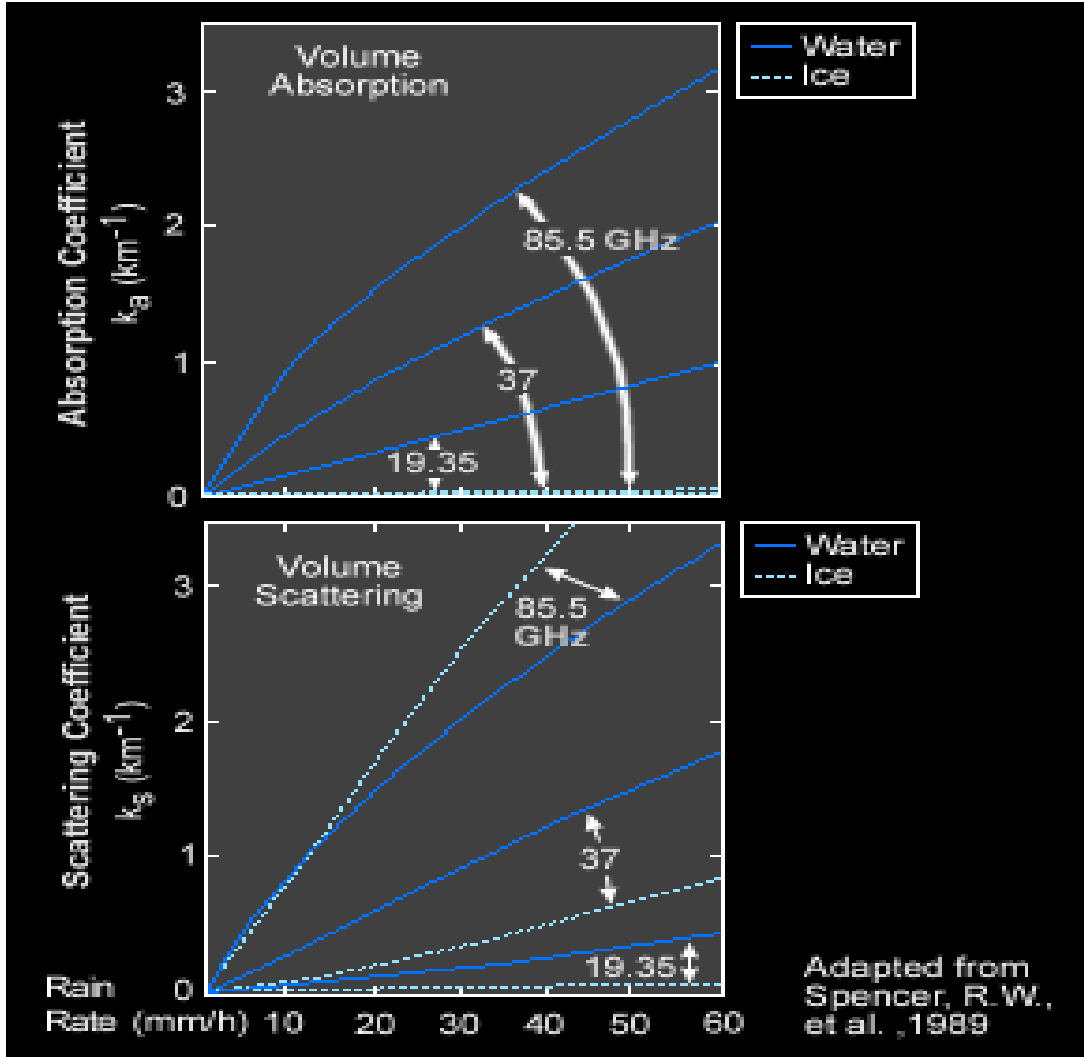
Figure 12.1 Volume absorption (top) and scattering coefficients (bottom) calculated with Mie theory for the Marshall-Palmer precipitation size distribution of water and ice spheres at three frequencies 19.35, 37, 85.5 GHz).
