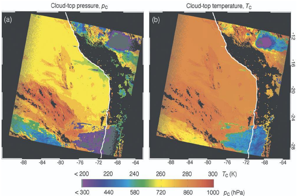
Figure 12.6 (a) Cloud-top pressure and (b) temperature retrievals for the image of Fig. 13.5 (from Platnick et al., 2003)
