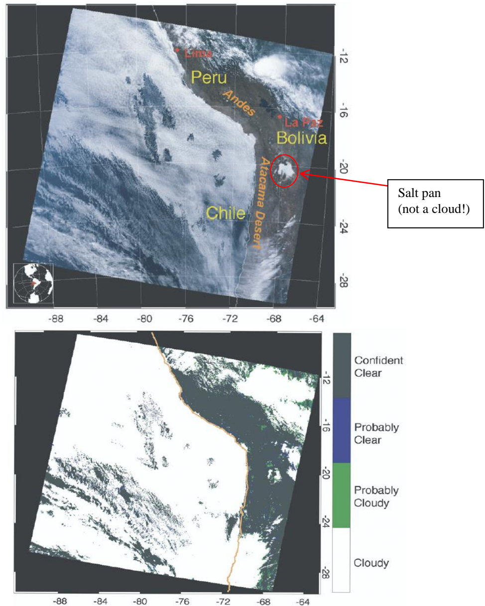
Figure 12.5 True-color image ( upper panel ) of a granule of Terra MODIS data from July 18, 2001, 1530 UTC. The image shows widespread boundary layer stratocumulus clouds off the coasts of Peru and Chile, associated with cool upwelling water along the Humboldt current. Over land clouds overly a variety of surfaces, including coastal deserts, high-altitude ecosystems, and low-land rain forests. Lower panel : retrieved cloud mask.
