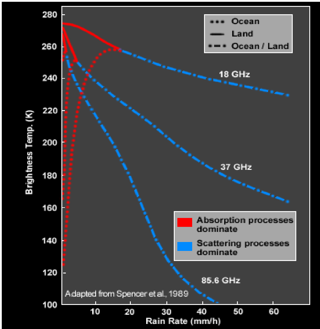
Figure 12.2 Brightness temperature vs. rain rate for three frequencies.
