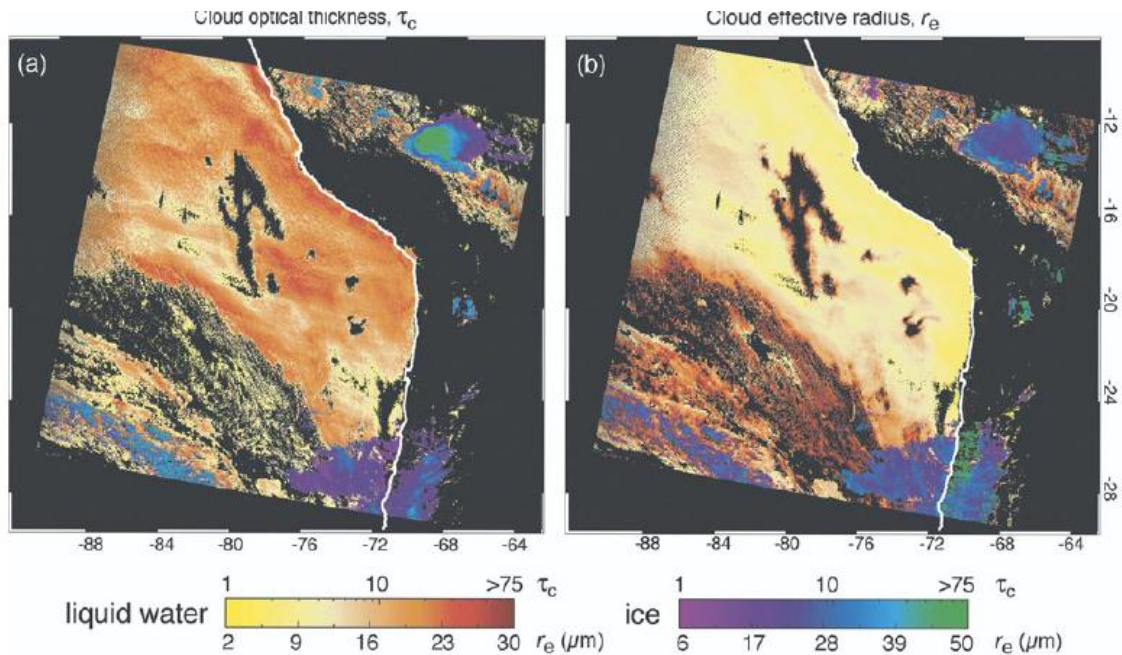
Figure 12.10 (a) Cloud optical thickness and (b) effective particle radius retrievals for the image of Fig. 13.5, with separate color bars for liquid water and ice clouds. Retrievals use the MODIS 2.1- \mu\text{m} band in conjunction with the 0.65- \mu\text{m} band (over land) and the 0.86- \mu\text{m} band (over water) (from Platnick et al., 2003).
