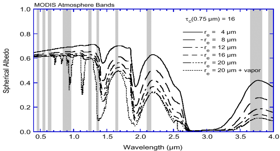
Figure 12.3 Cloud spherical albedo (reflectance) as a function of wavelength for selected values of the effective radius of cloud droplet. Computations were done for a water cloud having a modified gamma size distribution with an effective variance 0.111, cloud optical depth \tau_c(0.75 \mu\text{m})=16 , and water vapor content 0.45 \text{ g cm}^{-2} (ATBD MODIS cloud products). NOTE: spherical albedo is defined as F_{dif}^{\uparrow}(0)/\mu_0 F_0
