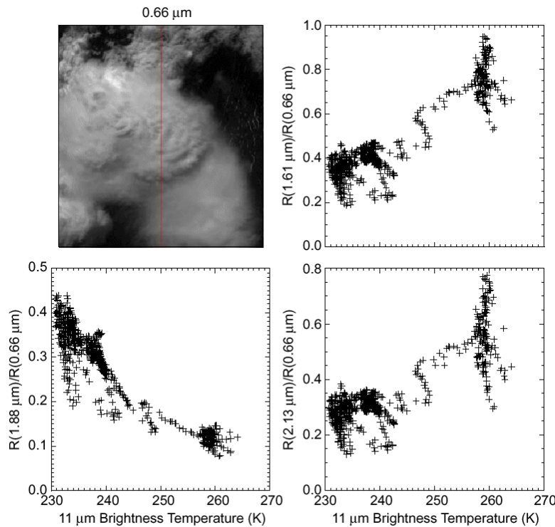
Figure 12.7 The upper left-hand panel shows the 0.66 image from MAS (MODIS airborne simulator) of a convective cumulonimbus cloud surrounded by lower-level water clouds. Subsequent panels show plots of the reflection function ratios as a function of corresponding BT at 11.02 \mu\text{m} . Nadir observations. The MAS 1.88 \mu\text{m} band is the analog for the MODIS 1.38 \mu\text{m} band (King et al., Cloud retrieval algorithm for MODIS). NOTE: Ice cloud: low reflectance at 1.61 and 2.13 \mu\text{m} and high reflectance at 1.88 \mu\text{m}
