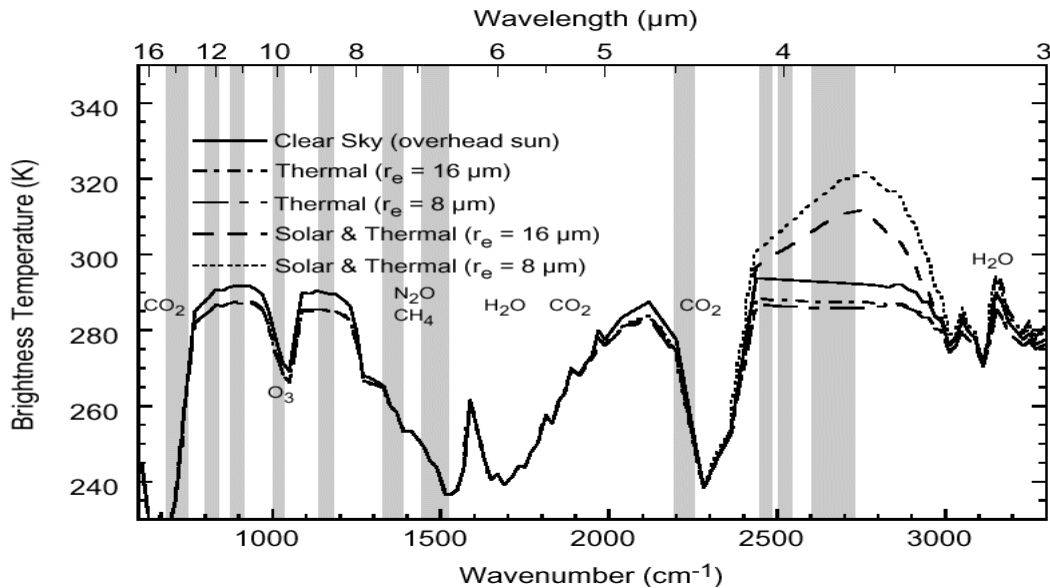
Figure 12.4 Brightness temperature as a function of wavelength (and wavenumber) for nadir observations and selected values of the effective radius of cloud droplets, cloud optical depth \tau_c(0.75 \mu\text{m})=5 for all cases. Computations were done for a water cloud having a modified gamma size distribution for the mid-latitude summer atmosphere with cloud top temperature T_{ct}=14 \text{ C} , cloud base temperature T_{cb}=17 \text{ C} , and blackbody surface temperature T_{sur}=21 \text{ C} .
