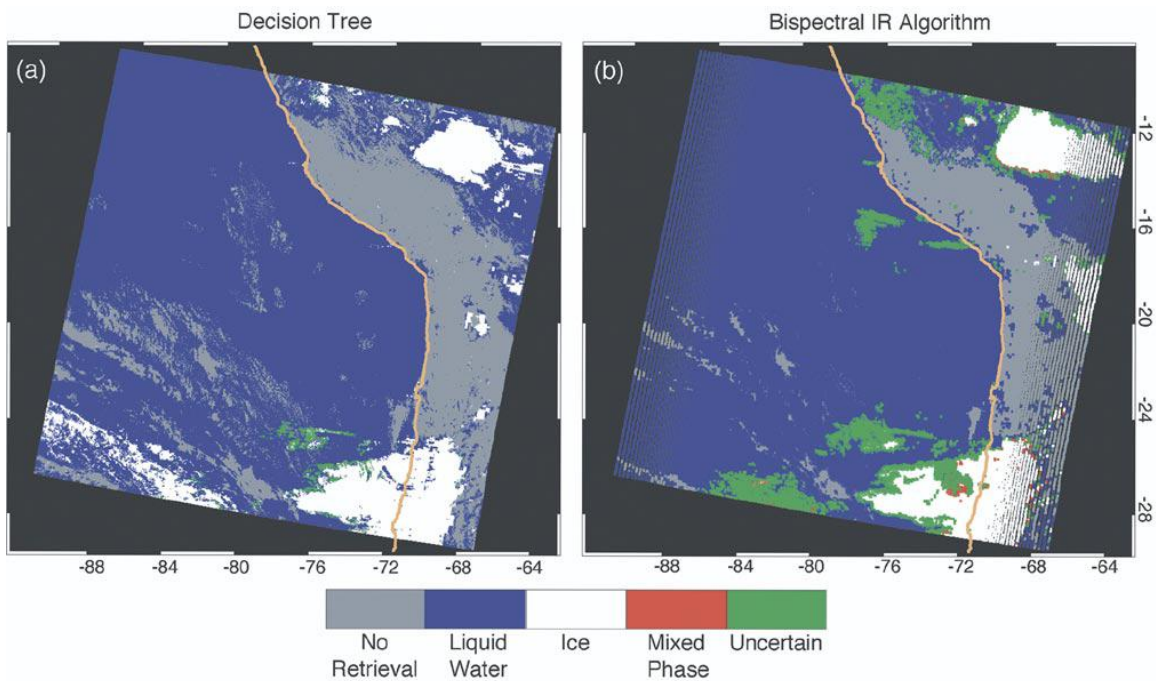
Figure 12.8 Two methods for retrieving cloud thermodynamic phase for the image of Fig. 12.6. (b) Results from the bispectral IR algorithm (8.5- and 11- \mu\text{m} MODIS bands).
