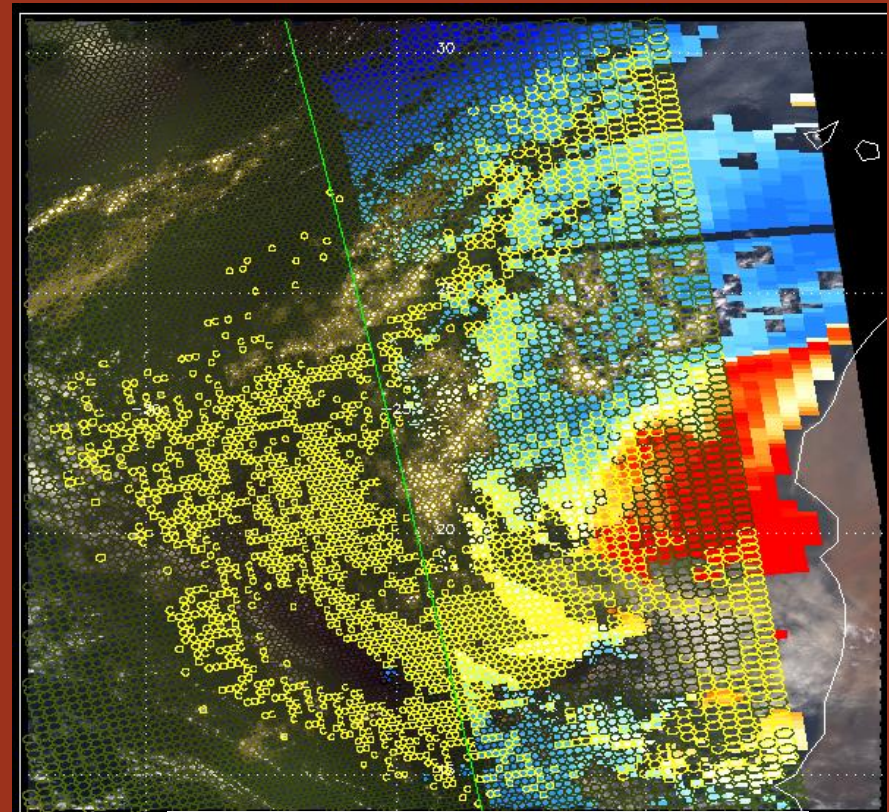
Collocated MODIS AOD and AIRS dust flag
