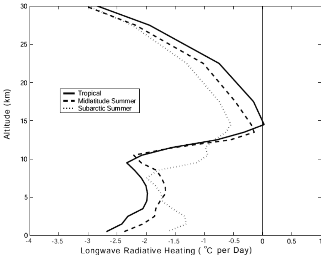
Figure 11.2 The total IR heating rates profiles calculate for three different model atmospheres.
