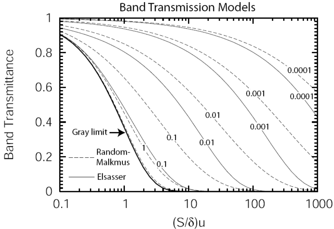
Figure 10.3 Comparison of the Elsasser (solid) and random-Malkmus (dashed) band models for several values of \gamma = \alpha/\delta (labeled on curves). For both models, curved approach the gray limit (Beer's law) when \gamma \gg 1 .
