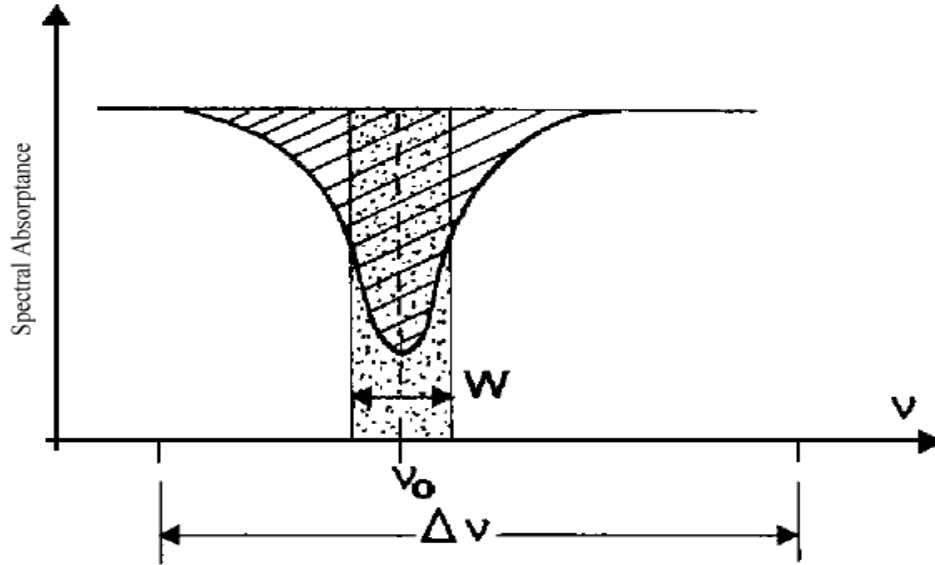
Figure 10.1 Schematic illustration of the equivalent width. The dotted rectangular area is equal to the hatched area and represents the total energy absorbed in the line.
