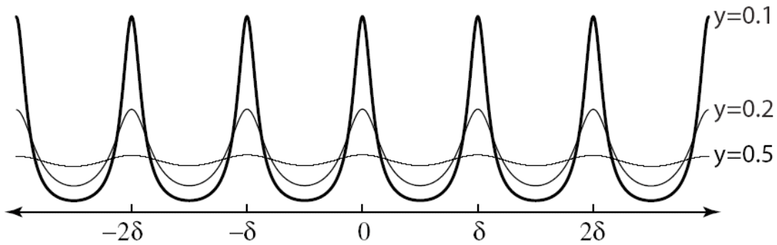
Figure 10.2 Schematic depiction of the absorption coefficient in the Elsasser (regular) band model, for three different values of y = \alpha/\delta .
