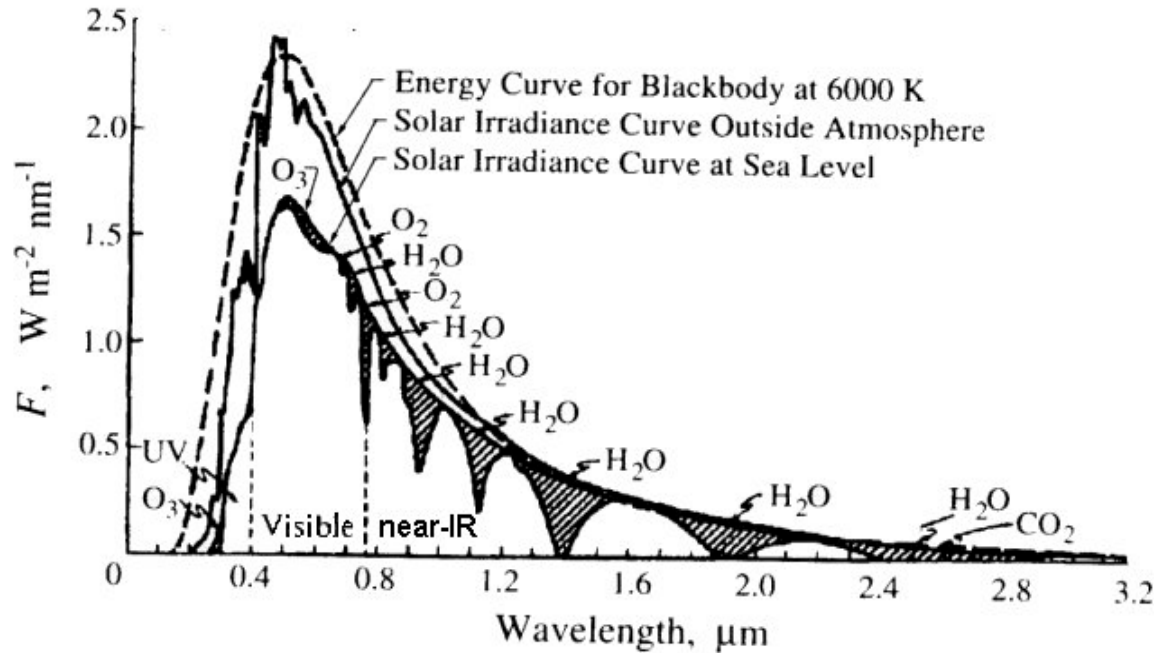
Figure 4.9 Solar spectral irradiance (flux) at the top of the atmosphere and at the surface.
