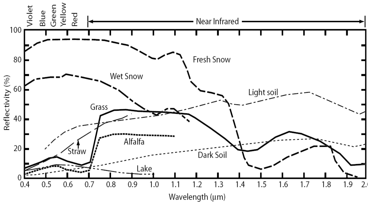
Figure 21.2 Typical shortwave spectral reflectances of various natural surfaces.
