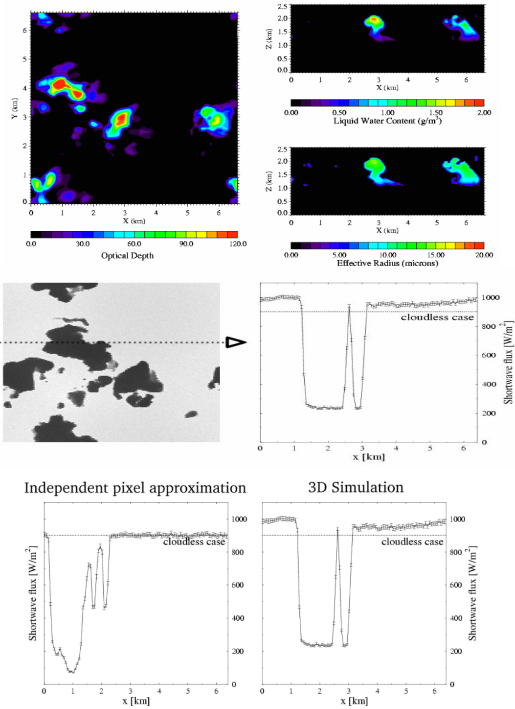
Figure 21.5 Solar flux ( 0.2\mu\text{m} - 4\mu\text{m} ) at the Earth's surface calculated with ICA and Monte Carlo for the cloud field shown on the upper panels. The sun is shining from the left, solar zenith angle is 30^\circ . The right image shows a cross section along the dotted line (Mayer et al).
