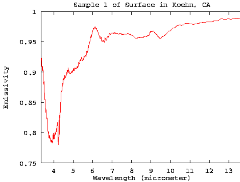
Figure 21.3 Examples of spectral emissivity (MODIS UCSB Emissivity Library)
