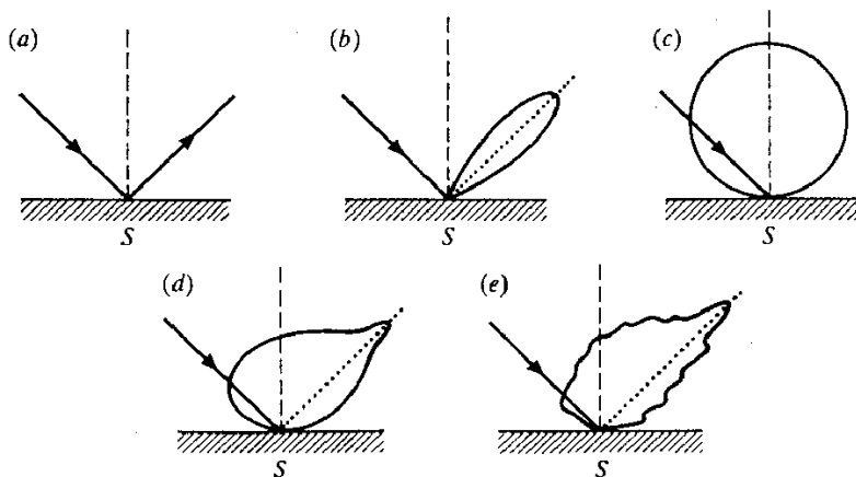
Figure 21.1 Schematic illustration of different types of surface scattering. The lobes are polar diagrams of the scattered radiation: (a) specular, (b) quasi-specular, (c) Lambertian, (d) quasi-Lambertian, (e) complex.
