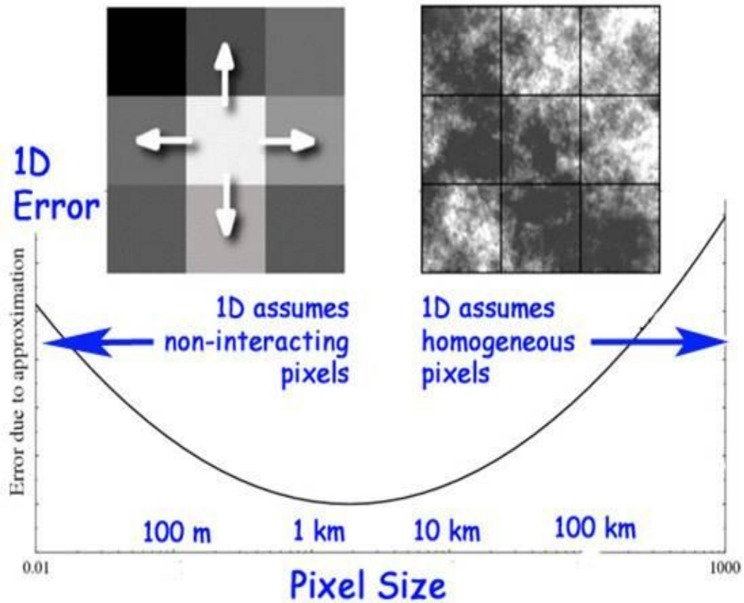
Figure 21.4 Illustration of the sources of errors in one-dimensional radiative transfer in cloudy conditions.
