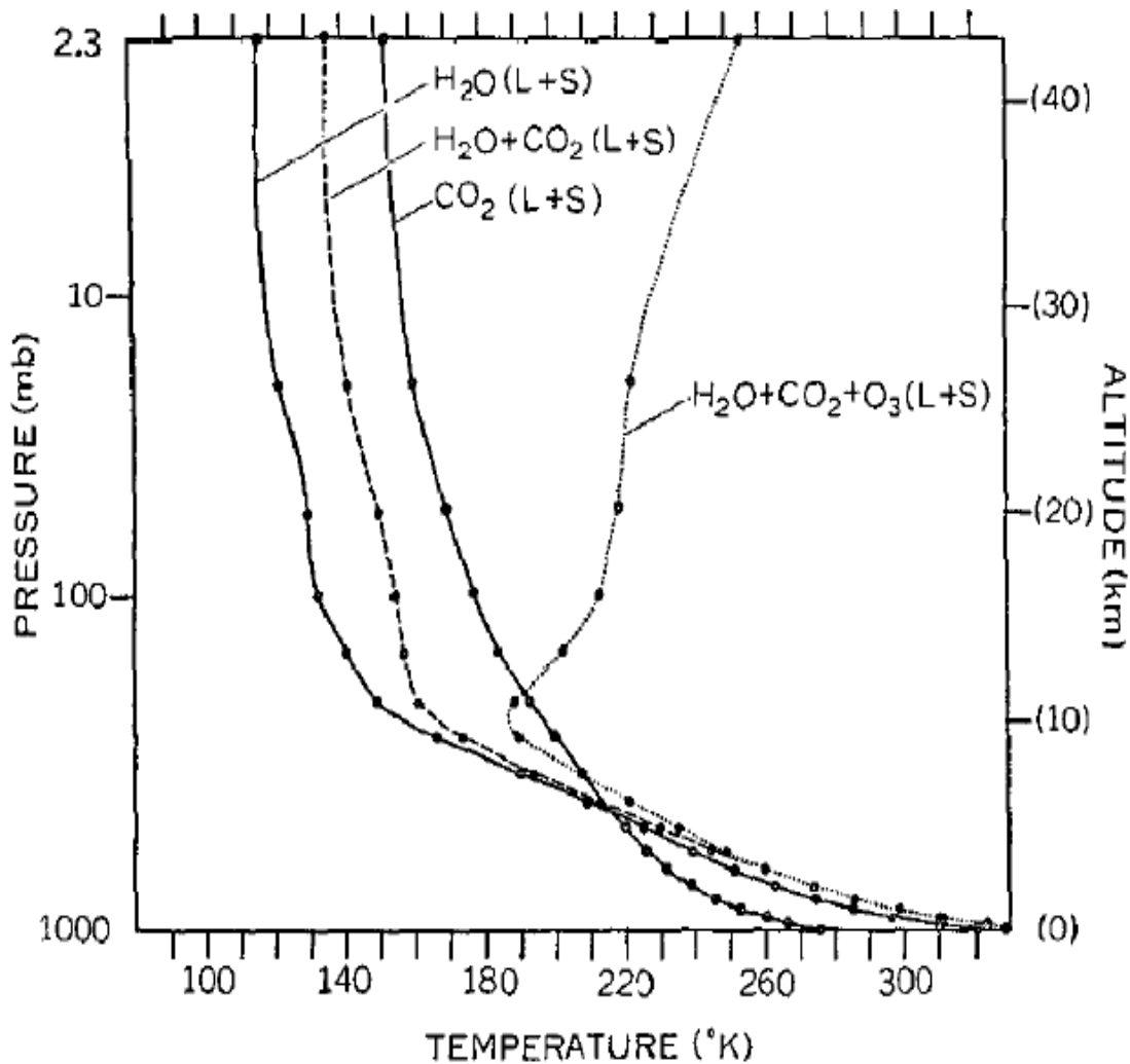
Figure 22.2 Pure radiative equilibrium temperature profiles for various atmospheric gases in a clear sky at 35 N in April. L+S means that the effects of both longwave and shortwave radiation are included (from Manabe and Strickler, 1964).
