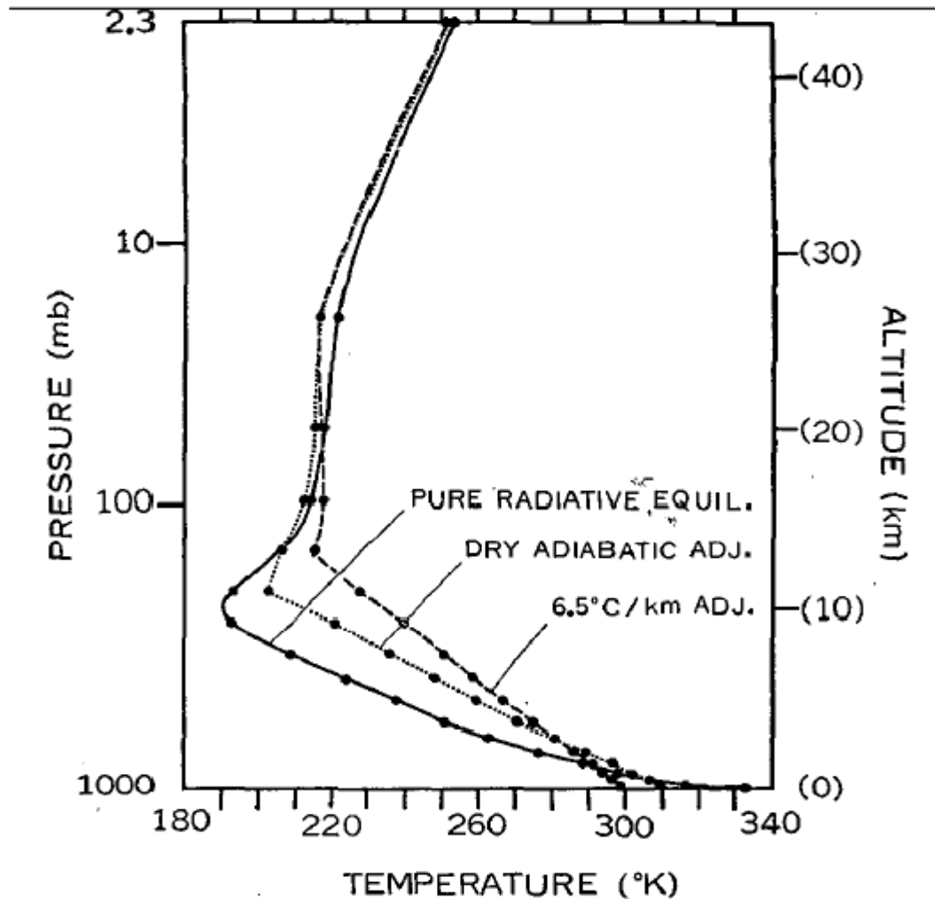
Figure 22.3 Pure radiative equilibrium and radiative-convective equilibrium temperature profiles for two values of \gamma_c for clear sky.
