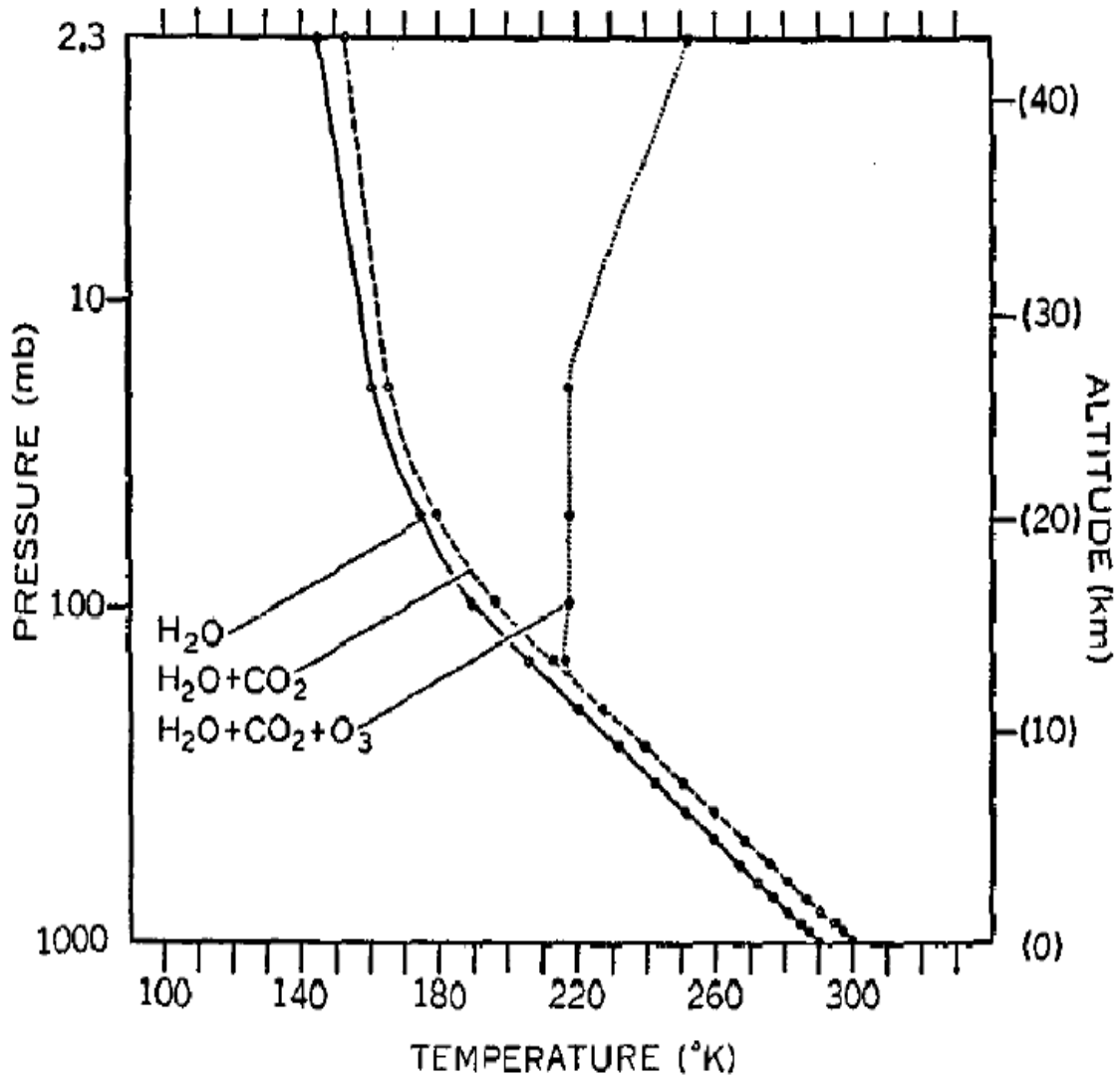
Figure 22.4 Radiative-convective equilibrium temperature profiles for various atmospheric gases in a clear sky at 35 N in April.
