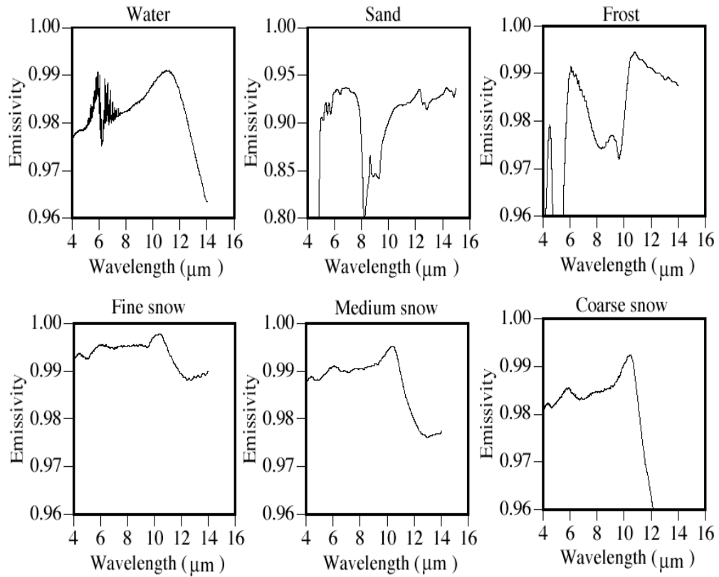
Figure 3.2 Examples of IR spectral emissivity of some surfaces.
