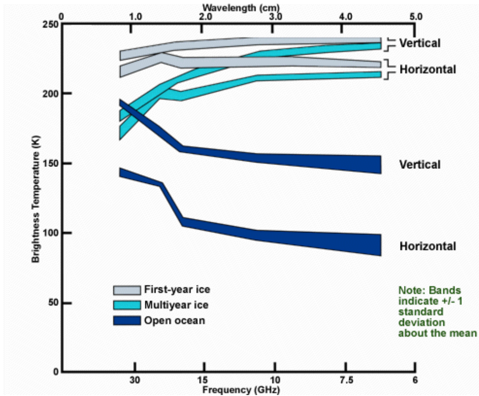
Figure 3.4 Microwave brightness temperature (at vertical and horizontal polarizations) as a function of frequency (wavelength) of first year sea-ice, multiyear sea-ice, and sea water as observed by the Nimbus-7 SMMR (Scanning Multichannel Microwave Radiometer) (Cavalieri et al., 1984).
