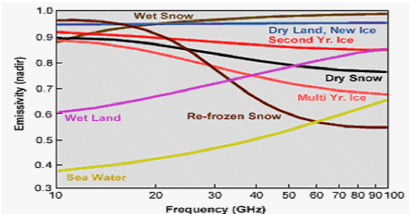
Figure 3.3 Examples of spectral emissivity (at nadir) of some surfaces in the microwave.
