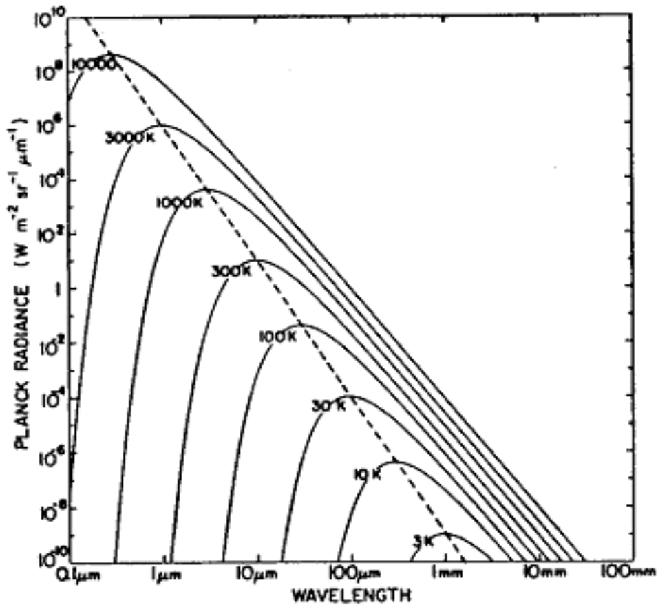
Figure 3.1 Planck function on log-log plot for several temperatures.
